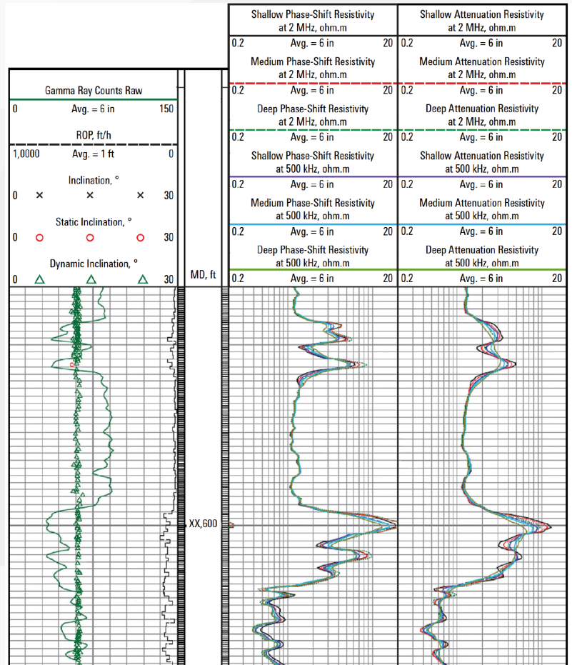
AWR Services provides high- and low-frequency curves through the pay section.
